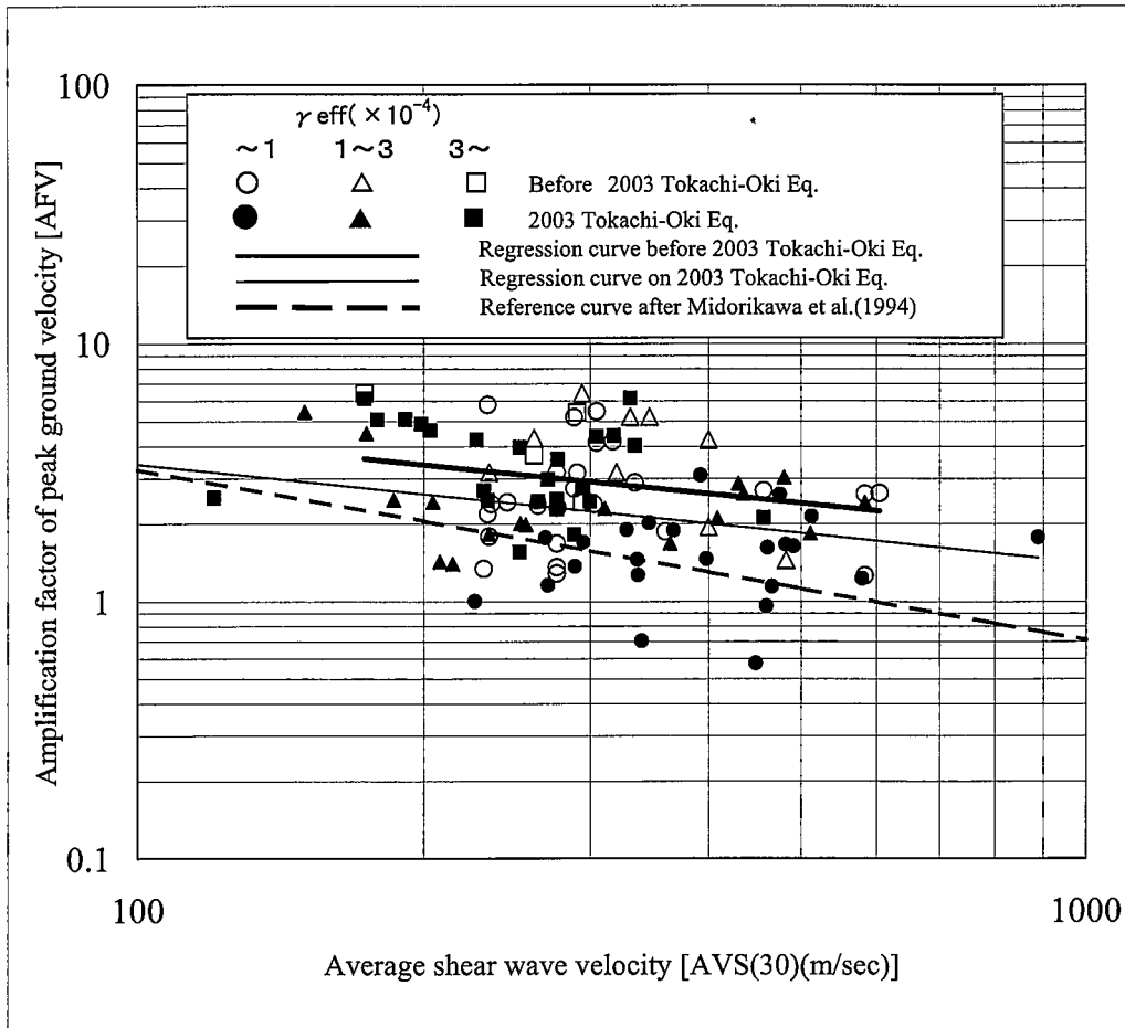
Fig. 5. Relation between the Amplification factors of the peak ground velocity (AFV) and the average shear wave velocity (AVS(30)).
