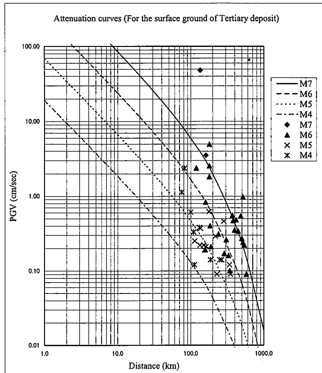
Fig. 3. Attenuation curves of the peak ground velocity (PGV) for the surface ground in the Tertiary deposit.
