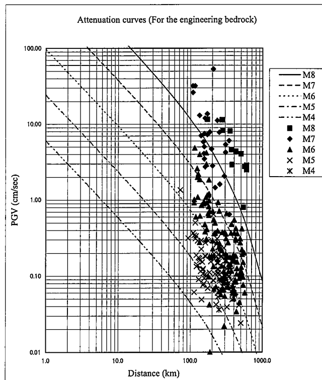
Fig. 4. Attenuation curves of the peak ground velocity (PGV) for the engineering bedrock.
